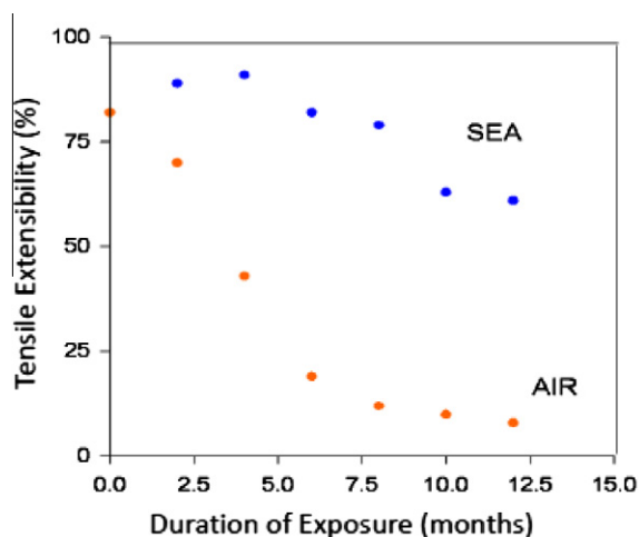
Fig. 2. (Left): Change in percent original tensile extensibility of polypropylene tape exposed in air and floating in sea water in Biscayne Bay, FL. (Right): The floating rig used to expose plastics to surface water environment (Miami Beach, FL).
