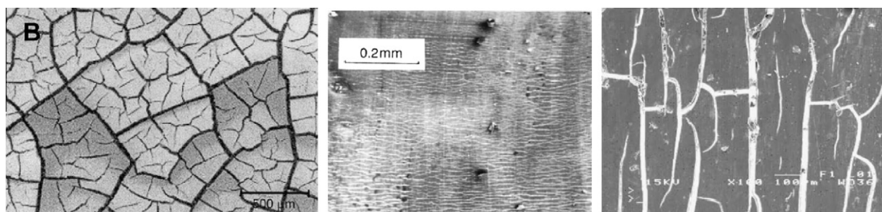
Fig. 4. Right: PP exposed to a 600 watt xenon source for 6 weeks (Yakimets et al. 2004); Middle: PP exposed for 1 week under desert exposure conditions (Qayyum and White, 1993); Left: LDPE weathered in a weatherometer for 800h (Küpper, et al., 2004).
